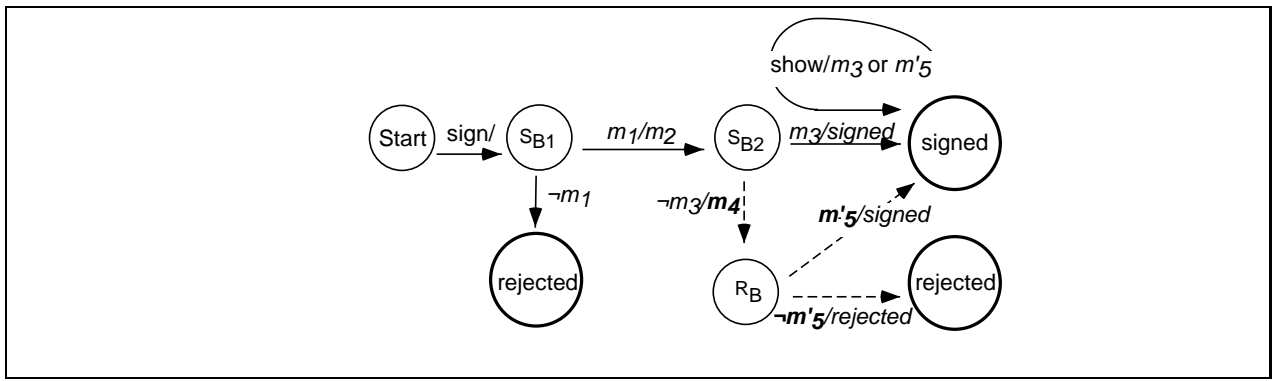
Figure 3: Signatory B of Scheme 1.
