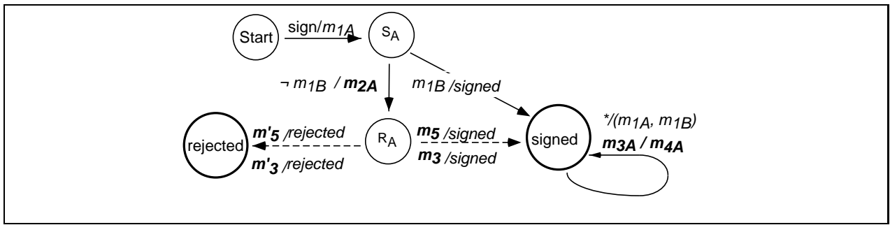
Figure 16: Signatory, e.g., A, of Scheme 5.
