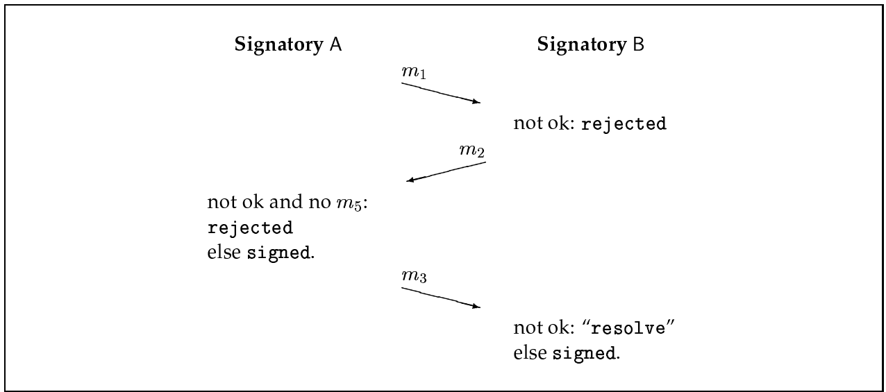
Figure 1: Optimistic Behavior of the Message-Optimal Synchronous Scheme 1.
