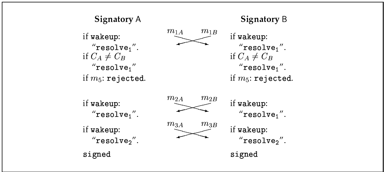
Figure 8: Optimistic Behavior of the Time-Optimal Asynchronous Scheme 3.
