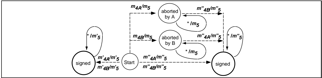
Figure 10: Third Party T of Scheme 3.
