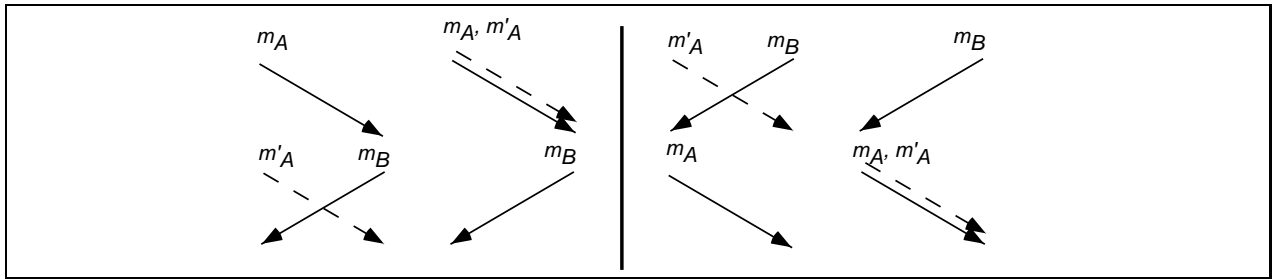
Figure 11: Proof of Theorem 3: Saving a Dashed Message by Shoving it Up or Down.
